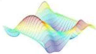
Mode 11: Deck Second Bending Mode (37.8Hz)
