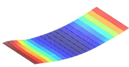
Mode 1: First Bending Mode (6.02 Hz)
