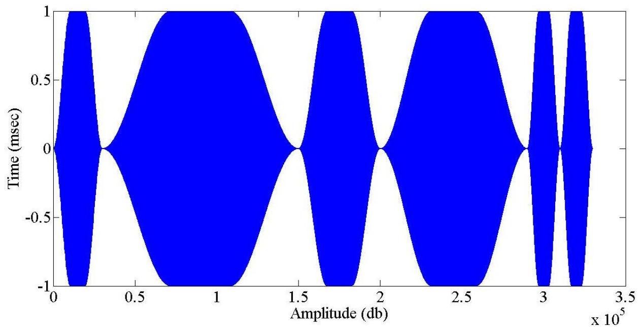
Figure 3.22 Time Domain of Tukey Windowed Targeted Sine Sweep Signal.
